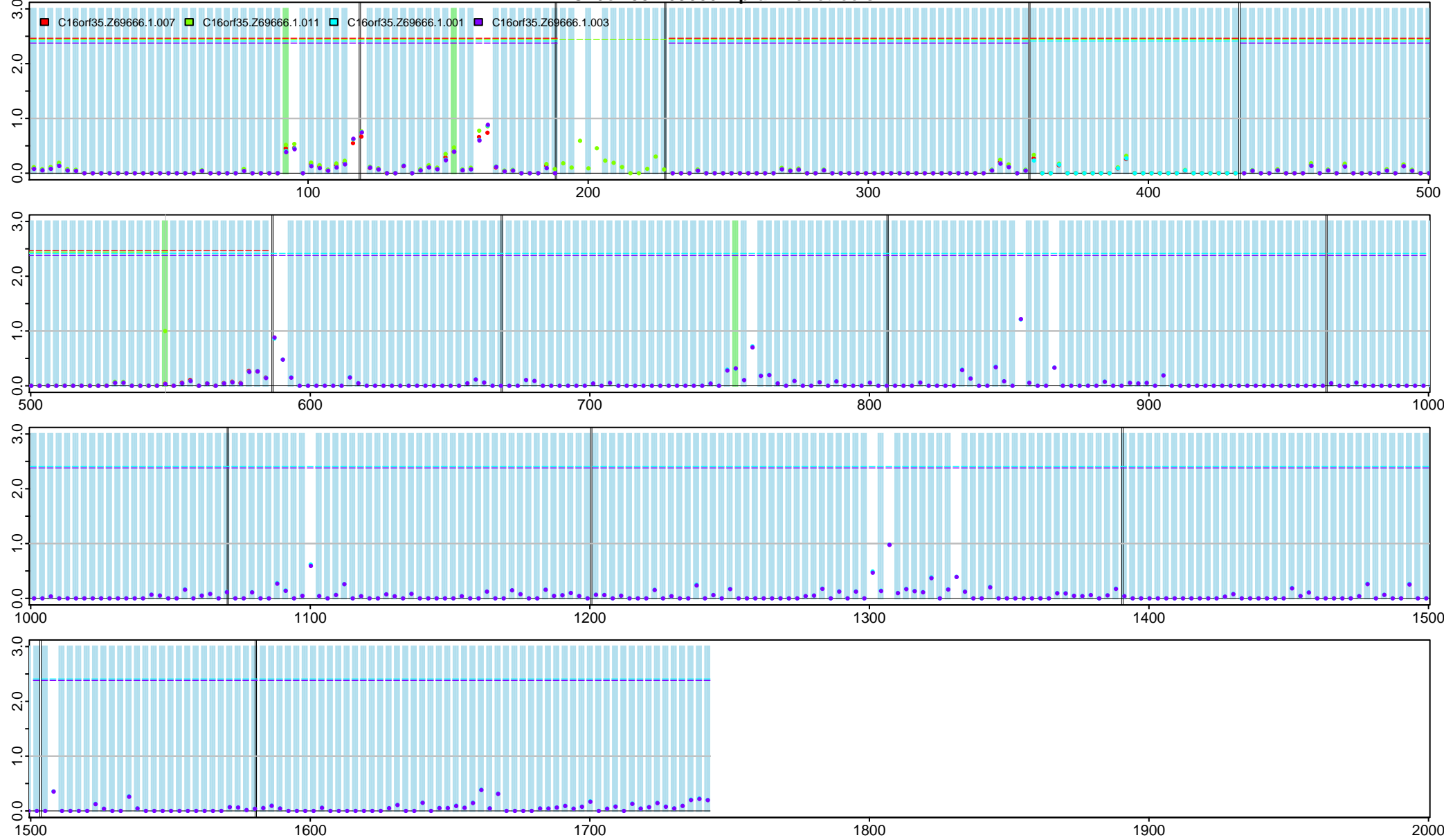
C16orf35.Z69666.1.prank.entree.slr
