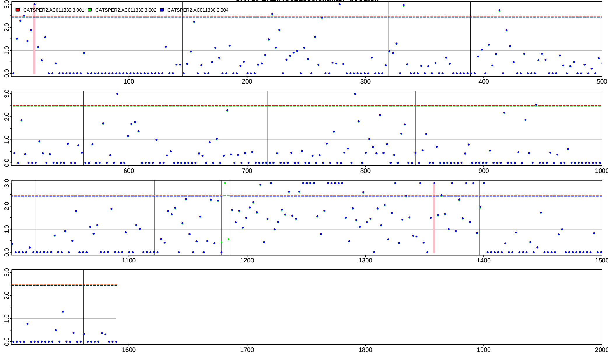
CATSPER2.AC011330.3.lagan good.slr
