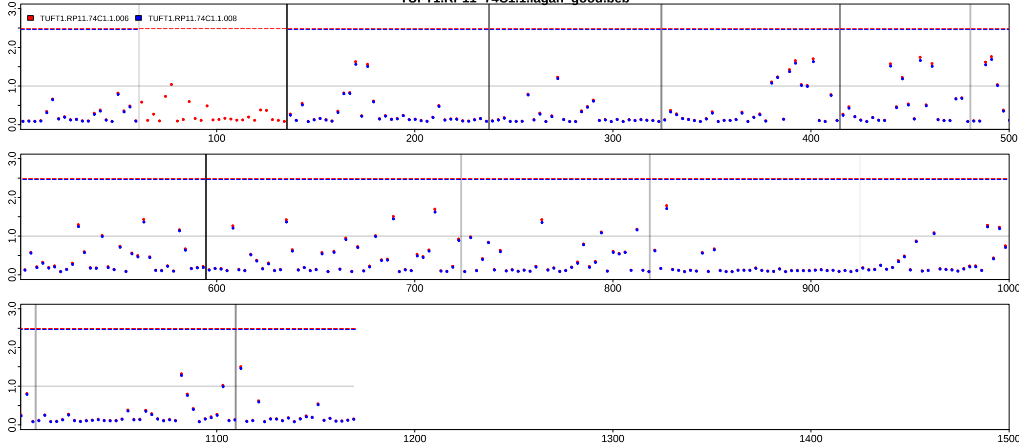
TUFT1.RP11-74C1.1.lagan_good.beb
