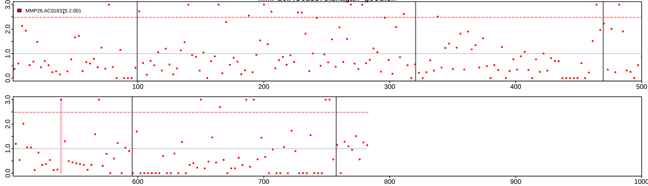
MMP26.AC018375.2.lagan_good.slr
