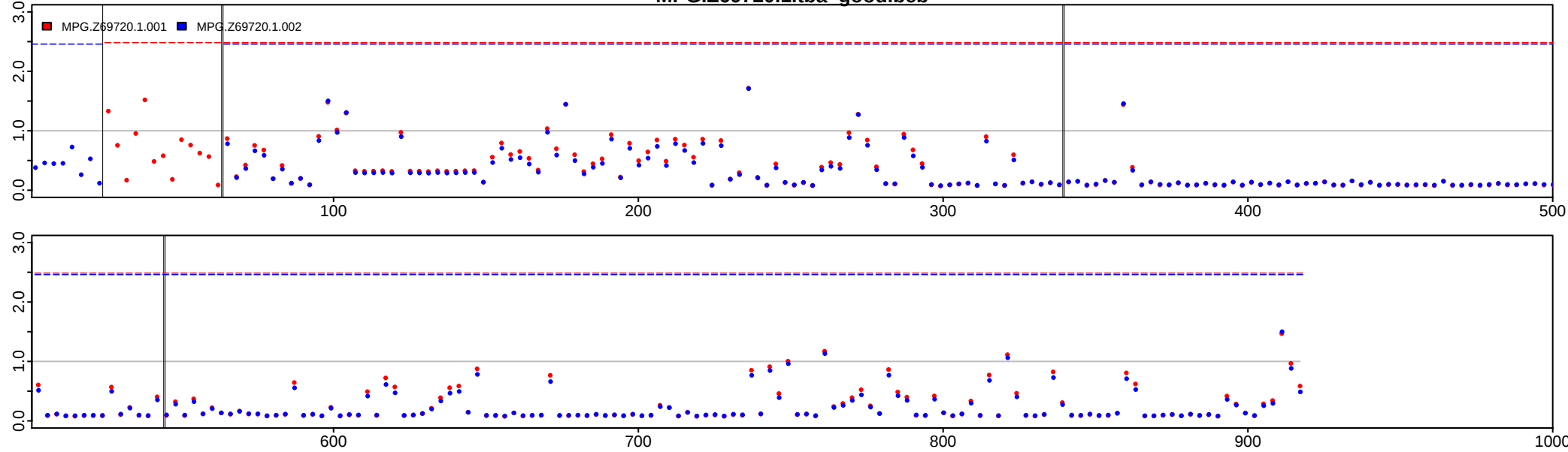
MPG.Z69720.1.tba good.beb
