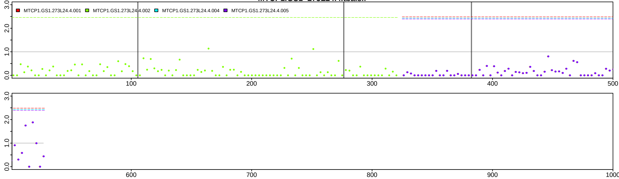
MTCP1.GS1-273L24.4.tba.slr
