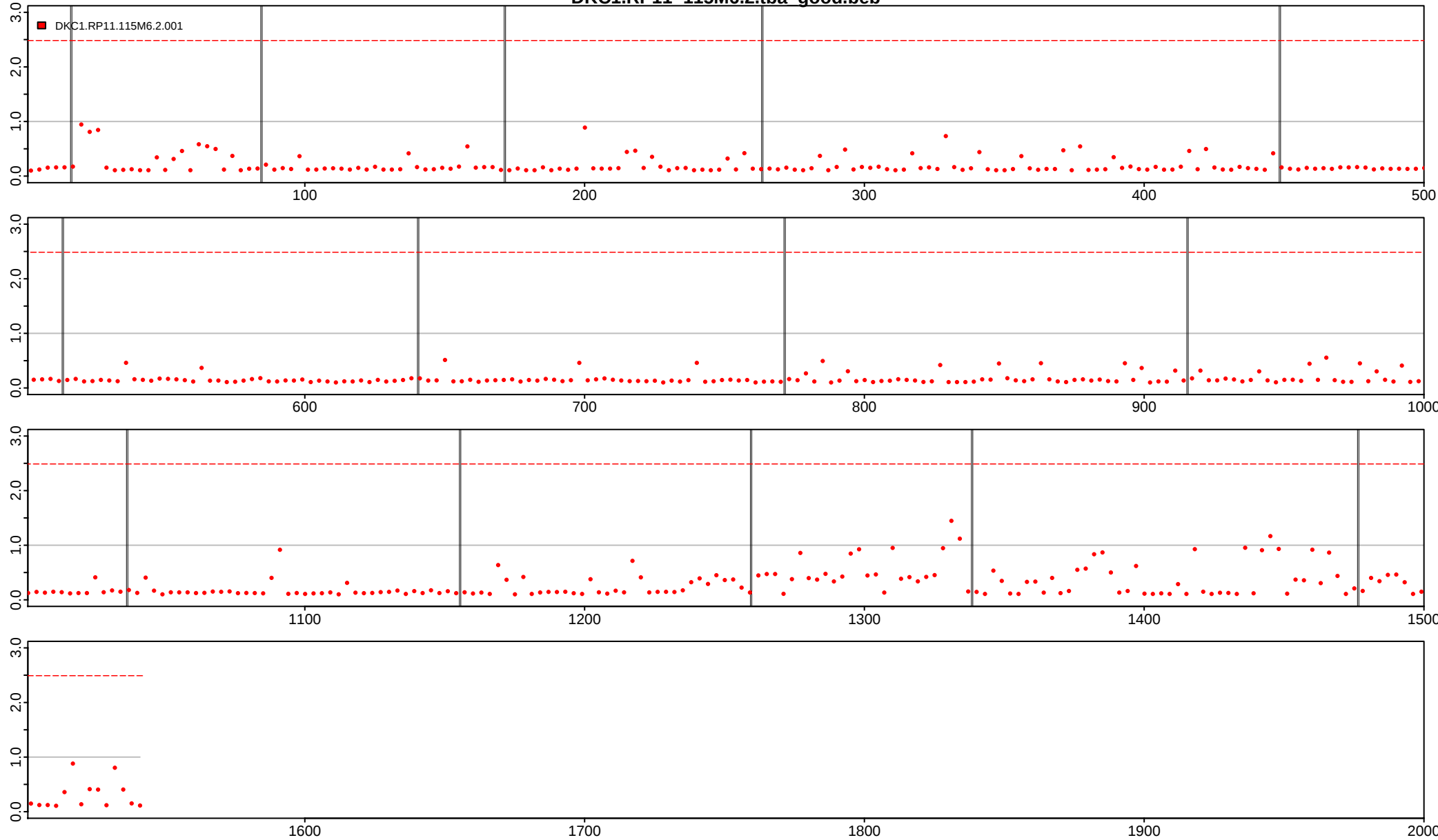
DKC1.RP11-115M6.2.tba good.beb
