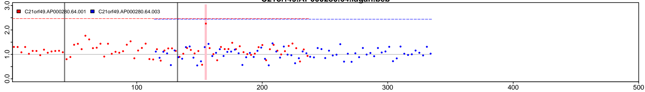
C21orf49.AP000280.64.lagan.beb
