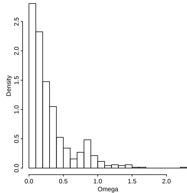
mean Ka/Ks: tba_good (n=726)
