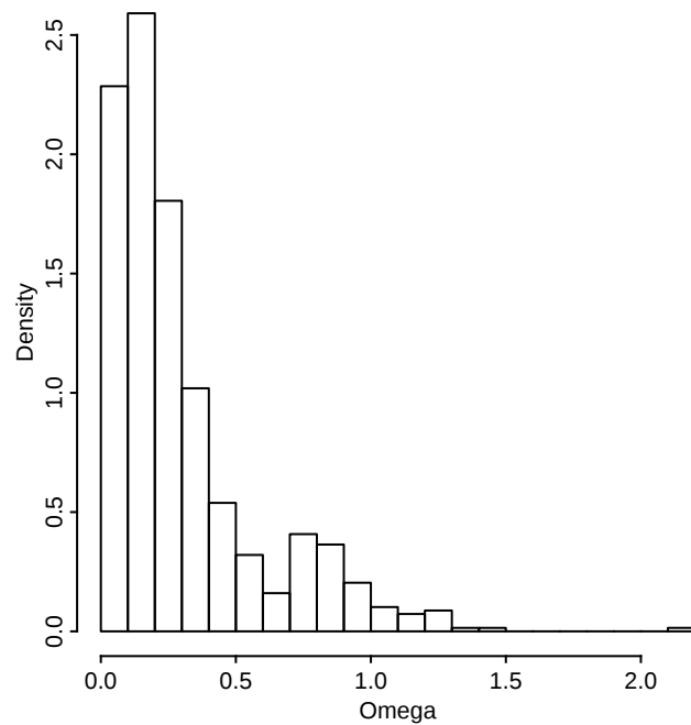
mean Ka/Ks: tba_mammals (n=726)
