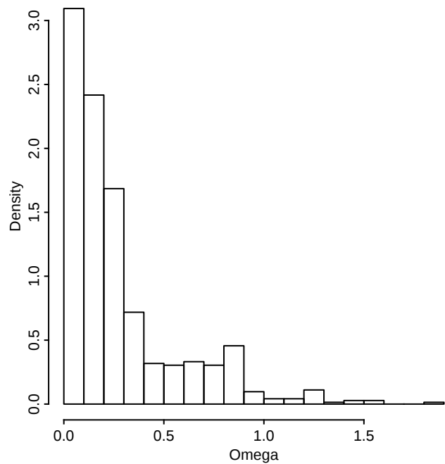
mean Ka/Ks: tba (n=726)
