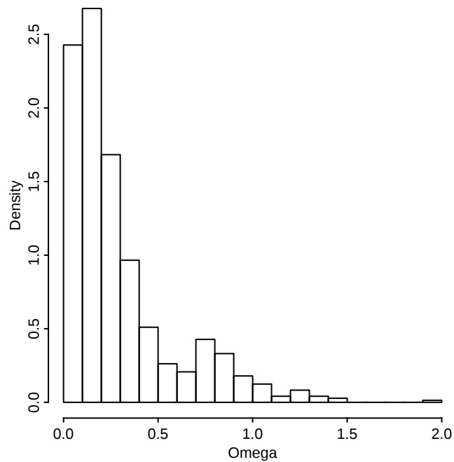
mean Ka/Ks: tba (n=726)
