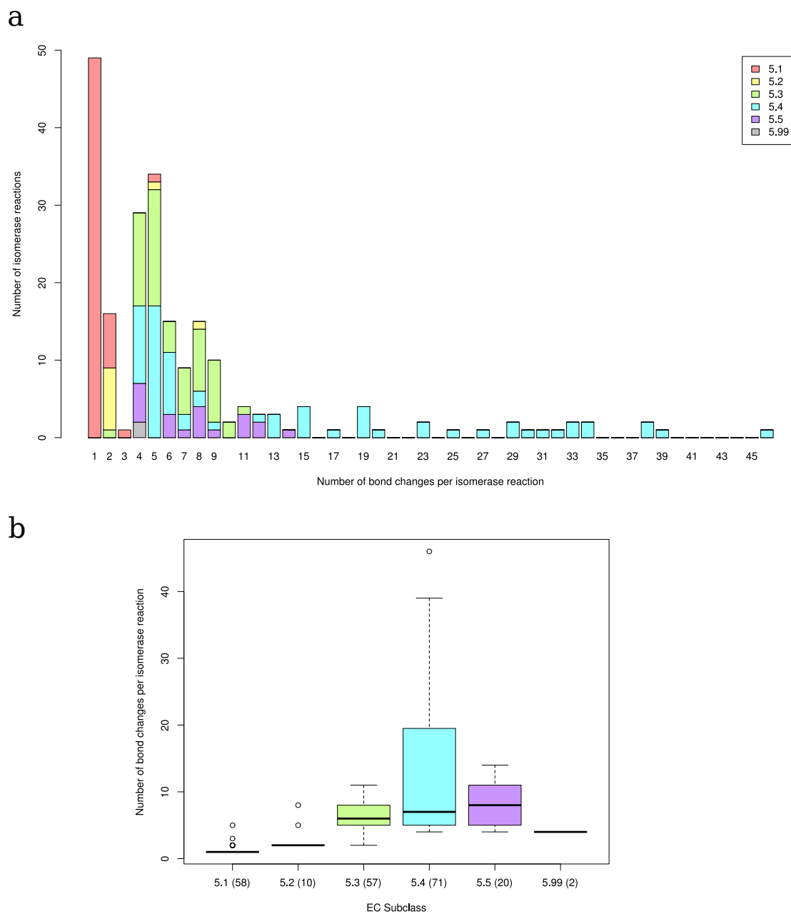
Figure 3.2: Distribution of the number of bond changes per isomerase reaction by EC subclass. (a) Bar plot showing the number of isomerase reactions against number of bond changes. (b) Box and whisker plot representing the distribution of the number of bond changes per isomerase reaction by EC subclass. The number of reactions belonging to each subclass is shown in brackets. Coloured boxes contain the interquartile range of each subclass. Whiskers represent 1.5 times the size of the coloured boxes. Single points beyond the whiskers represent outliers (Crawley, 2007).
