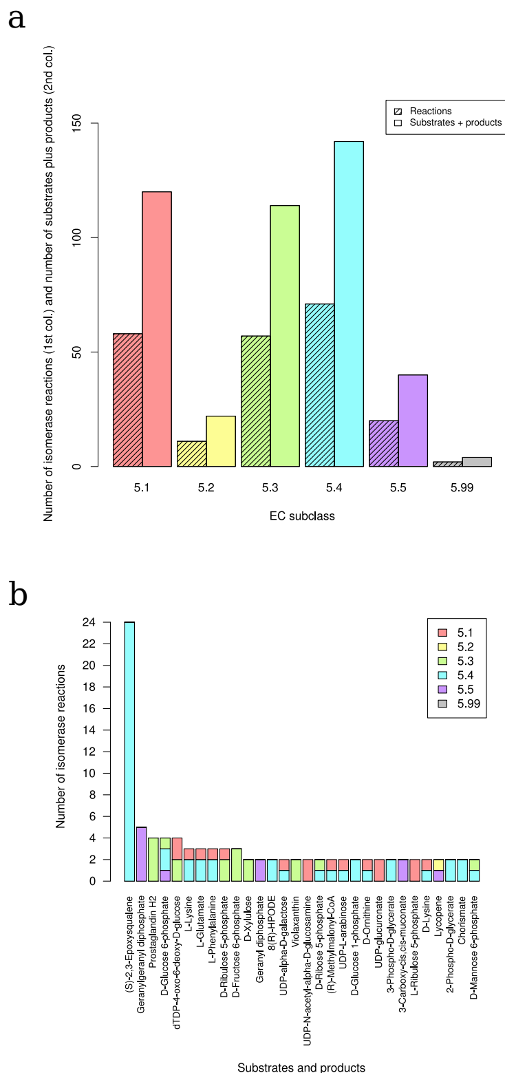
Figure 3.10: Distribution of substrates and products in isomerase reactions. (a) Distribution of the 442 occurrences of substrates and products in 219 representative isomerase reactions across EC subclasses (b) Bar plot showing the distribution of the 30 most common compounds present as substrates or products in isomerase reactions.
