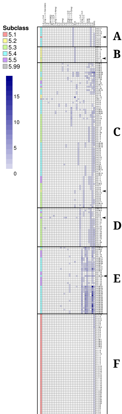
Figure 3.5: Hierarchical clustering of isomerase reactions (rows) by bond changes (columns). The blue scale represents frequency of bond changes in reactions. Reactions are annotated in colours according to their EC subclass (left-hand column). Six clusters were identified (A to F) (see Figure 3.4b). Bond changes were ordered left-to-right according to increasing frequency (Figure 3.3). Outliers are annotated with an arrow (see main text).
