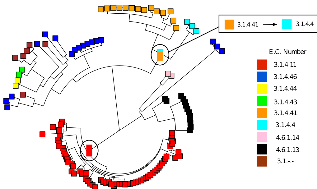
Figure 2.8: (a) Illustration of the FunTree pipeline (b) Example of the estimation of a functional change during the evolution of PIP superfamily. Phospholipase D activity (EC 3.1.4.4, cyan) was inferred to have evolved from sphingomyelin phosphodiesterase D activity (EC 3.1.4.41, orange). Image courtesy of Dr. Nicholas Furnham.
