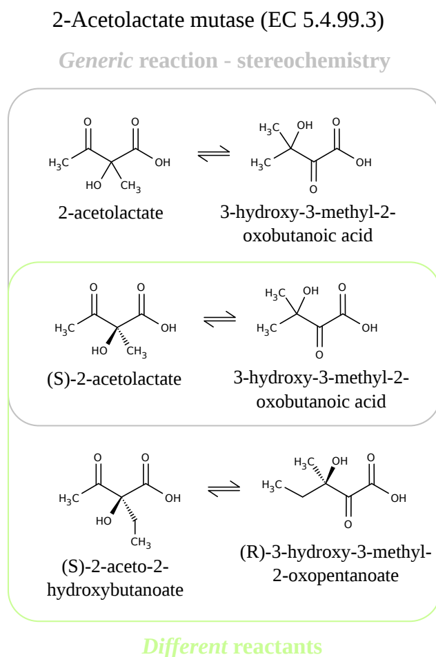
Figure 5.3: 2-Acetolactate mutase (EC 5.4.99.3) is an example of EC number assigned to two groups of reaction diversity: different types of reaction and partial reactions.
